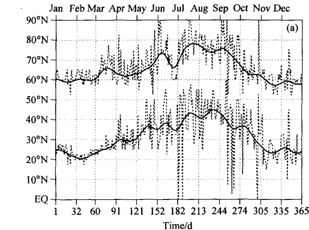
图 1 1948~2005 年北半球 (a) 和南半球 (b) 逐日纬向平均 SLP 各纬度之间交叉相关中最大负相关系数相对应的两个纬度的年变化。粗实线: 31 天 Gauss 平滑序列 Fig. 1 The annual variations of corresponding two latitudes with the biggest negative values of cross correlation coefficients of the daily zonal mean sea level pressures (SLPs) in the (a) Northern and (b) Southern hemispheres from 1948 to 2005. The solid line is 31-day Gaussian smooth series
