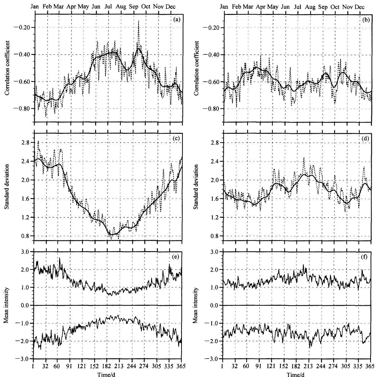
图2 1948~2005年 (a) 北半球和 (b) 南半球逐日纬向平均 SLP 各纬度之间交叉相关中最大负相关系数的年变化; (c) NAMI 和 (d) SAMI 逐日标准差年变化; (e) NAMI 和 (f) SAMI 正 (实线)、负 (虚线) 位相平均强度的年变化。(a~d) 粗实线为 31 天 Gaussian 平滑序列 Fig. 2 The annual variations of the biggest negative cross correlation coefficients of the daily zonal mean SLPs in the (a) Northern and (b) Southern hemispheres; the standard deviations of (c) the Northern Hemisphere Annual Mode Index (NAMI) and (d) the Southern Hemisphere Annual Mode Index (SAMi); (e) the mean intensity of positive phase (solid line) and negative phase (dashed line) of NAMI; (f) same as (e), but for SAMI. The solid lines in (a)~(d) are 31-day Gaussian smooth series
