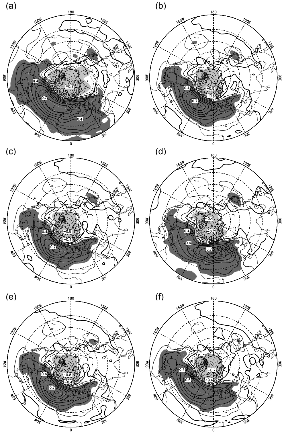
Fig. 2. Correlation coefficients between monthly SLP and (a) the NAOI, (b) NAOIR, (c) NAOIH, (d) NAOIJ, (e) NAOIM, and (f) NAOIB indices in the Northern Hemisphere for the period 1958–2000. The shading indicates significance at the 99.9% confidence level.
