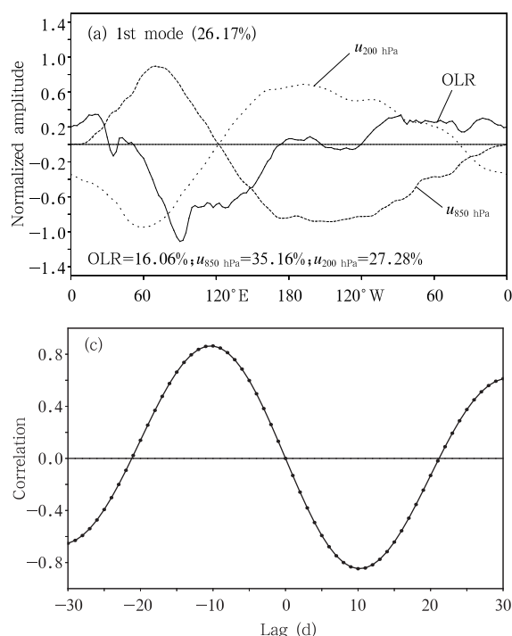
图7 OLR、850和200 hPa纬向风3个变量30—60 d滤波且15°S—15°N平均之后,联合EOF分析所得到的前两个空间模态的分布情况,以及前两个模态对应的时间系数PC1和PC2的超前滞后相关情况 (a. CEOF-1, b. CEOF-2, c. PC1和PC2的超前滞后相关曲线) Fig. 7 The first (a) and second (b) combined EOF (CEOF) modes of the 30–60 d filtered OLR, and the 850 and 200 hPa zonal winds averaged over 15°S–15°N, as well as the lead-lag correlation coefficients between them (c)
