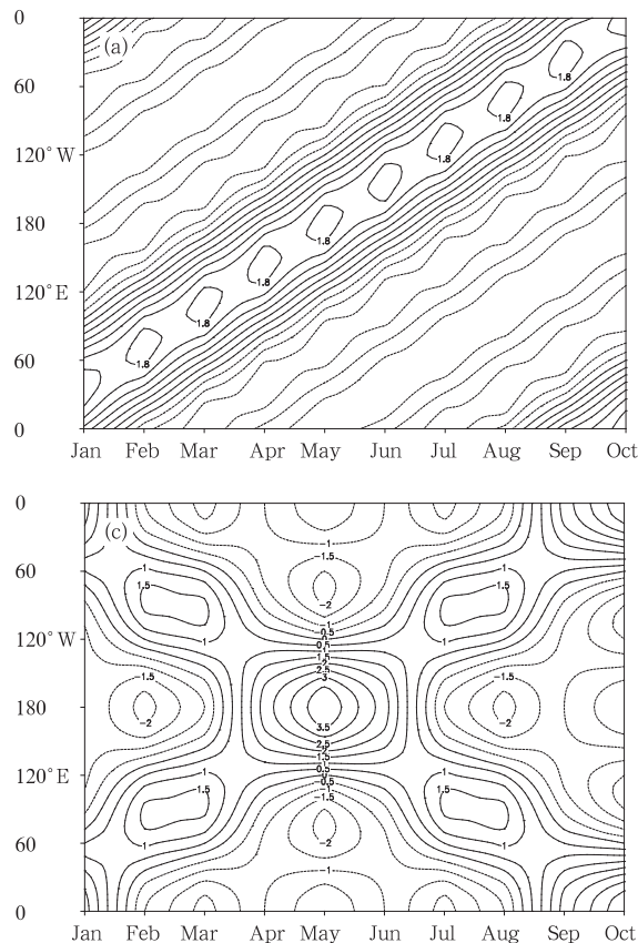
Fig. 4 As in Fig. 2 but for the time-space series F_1(x, t) .
