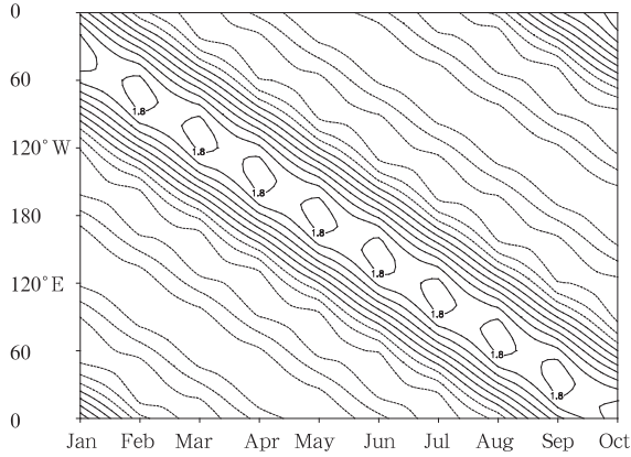
图 2 理想函数构造的单向传播的时-空序列 f(x, t) 经过时-空二维波传播分解后得到的随时间向西传播的分量的时-空分布 Fig. 2 Time-space cross section of the westward-propagating component derived via the Space-Time Wave Propagating Decomposition (STWPD) of the unidirectionally propagating time-space series f(x, t) , which is constructed by the ideal function
