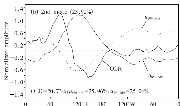
图7 OLR、850和200 hPa纬向风3个变量30—60 d滤波且15°S—15°N平均之后,联合EOF分析所得到的前两个空间模态的分布情况,以及前两个模态对应的时间系数PC1和PC2的超前滞后相关情况 (a. CEOF-1, b. CEOF-2, c. PC1和PC2的超前滞后相关曲线) Fig. 7 The first (a) and second (b) combined EOF (CEOF) modes of the 30–60 d filtered OLR, and the 850 and 200 hPa zonal winds averaged over 15°S–15°N, as well as the lead-lag correlation coefficients between them (c)
