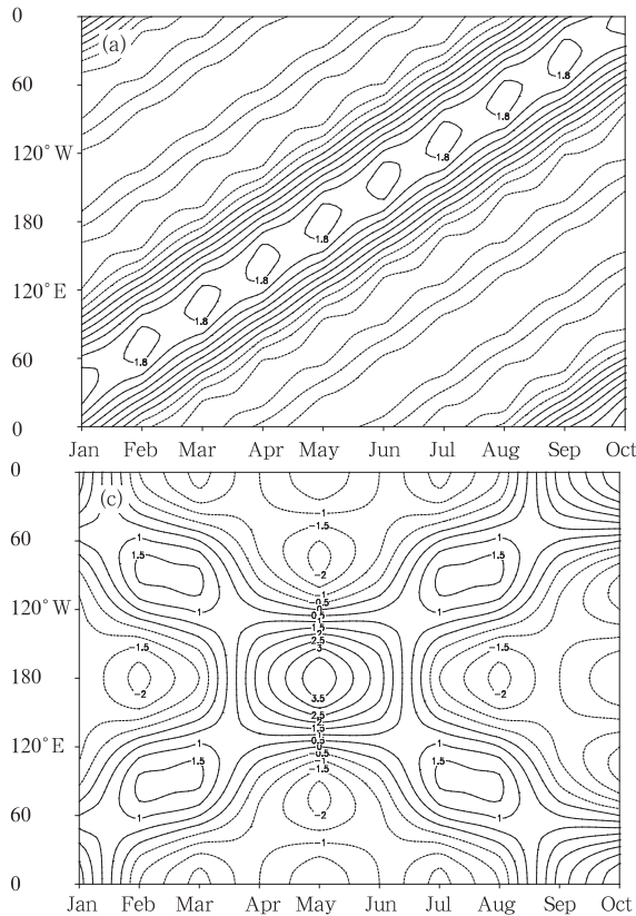
图 2 理想函数构造的单向传播的时-空序列 f(x, t) 经过时-空二维波传播分解后得到的随时间向西传播的分量的时-空分布 Fig. 2 Time-space cross section of the westward-propagating component derived via the Space-Time Wave Propagating Decomposition (STWPD) of the unidirectionally propagating time-space series f(x, t) , which is constructed by the ideal function
