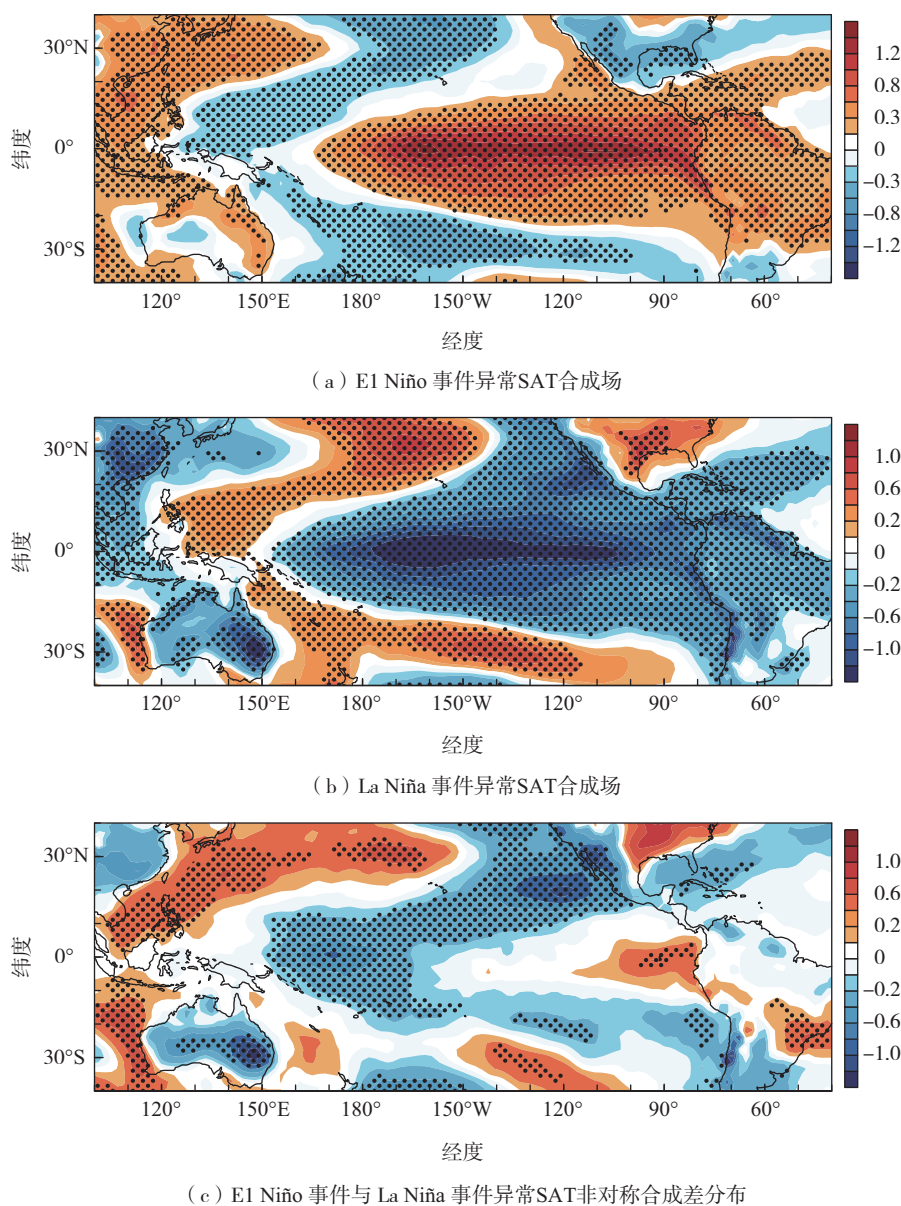
图 6 同图 3,但表示 2 m 高度上 SAT 异常场及其非对称空间分布 Fig.6 The same as Fig.3, but for spatial distribution of SAT anomaly at 2 m and its asymmetric spatial distribution
