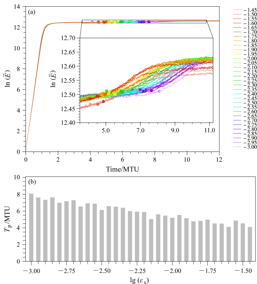
图2 在 \varepsilon_f=12 时,取不同 \varepsilon_s 值时快系统(a)相对误差的自然对数随时间增长曲线和(b)可预报时间( T_p ,单位:MTU)随 \varepsilon_s 的变化。图a的内插图为达到饱和时误差增长曲线的局部放大,圆点表示误差达到各自饱和值的时间点,下同。 \varepsilon_s 值的大小均以对数化后的 \lg(\varepsilon_s) 表示。 Fig. 2 (a) Temporal evolution of the natural logarithmic error growth and (b) the predictability limit ( T_p , units: MTU) of the fast dynamics with different values of slow coupling parameter \varepsilon_s and a constant value of fast coupling parameter ( \varepsilon_f=12 ). The inset of Fig. a is the enlarged detail of the error growth curve when the error reaches saturation, and the dots correspond to the positions where the respective error growth reaches saturation, the same below. The values of \varepsilon_s are indicated by logarithmicized [ \lg(\varepsilon_s) ].
