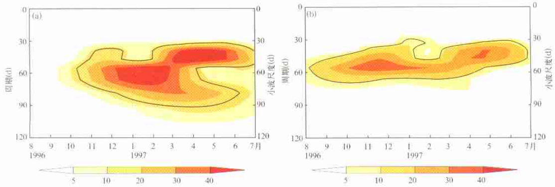
图3 EOF1和EOF2对应的时间系数 P_{1t} 和 P_{2t} 时间系数Morelet小波功率谱分析 (a. P_{1t} 小波分析功率谱, b. P_{2t} 小波分析功率谱; 粗实线包括区域表示通过时间滞后1, 相关系数为0.98的红噪音95%信度检验的区域) Fig.3 Local Morelet-wavelet power spectrum of (a) P_{1t} and (b) P_{2t} corresponding to the mode of EOF 1 and EOF2, (The left axis is the Fourier period (day) corresponding to the wavelet scale on the right axis. The solid line encloses regions of greater than 95% confidence level for a red-noise process with a lag=1 coefficient of 0.98)
